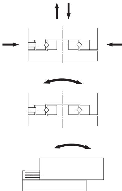
Fig.2 Load Directions
