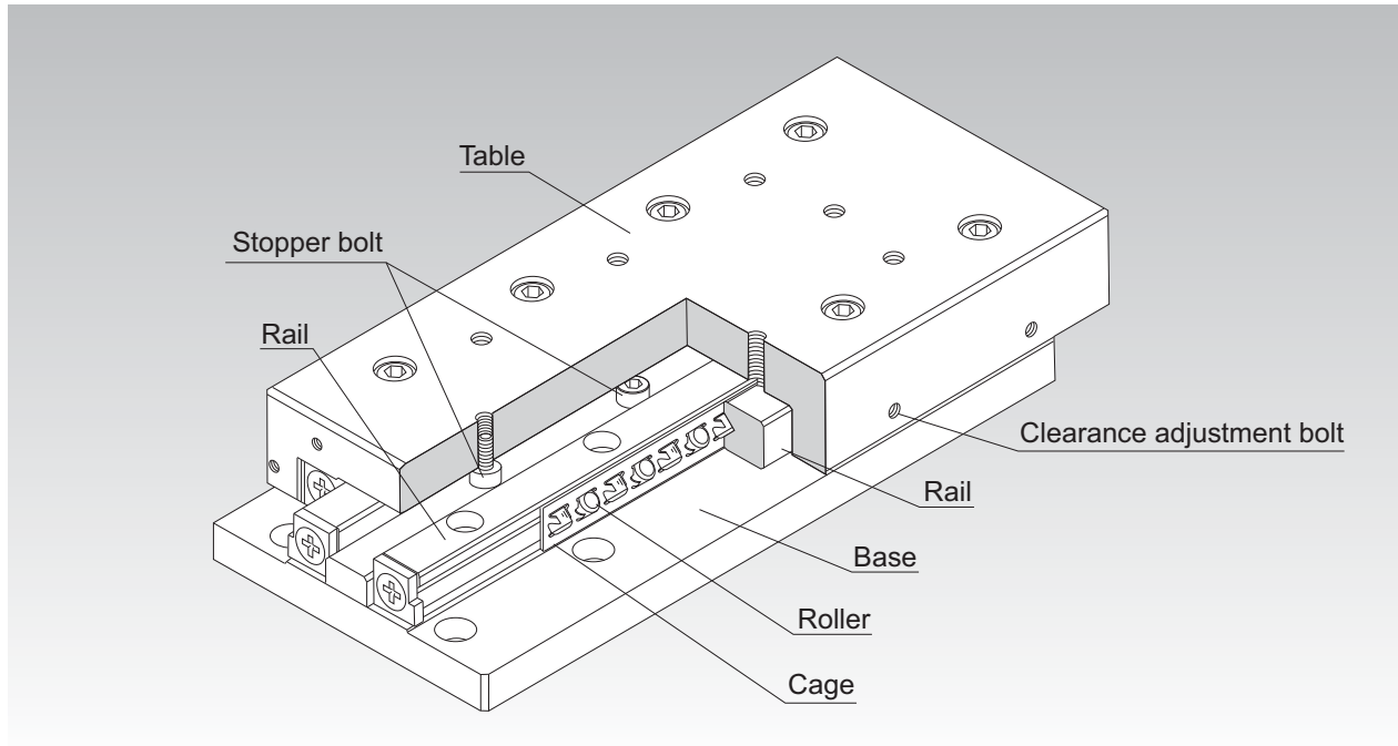
Fig.1 Structure of the Cross Roller Table
