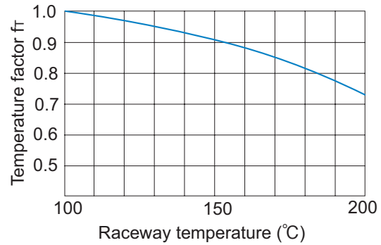
Fig.1 Temperature Factor (f T )
